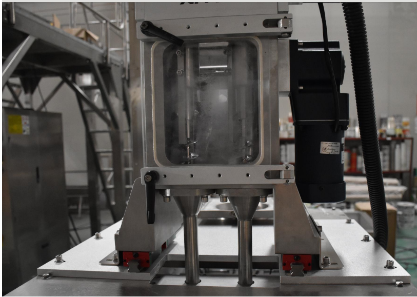
Auger/Screw
