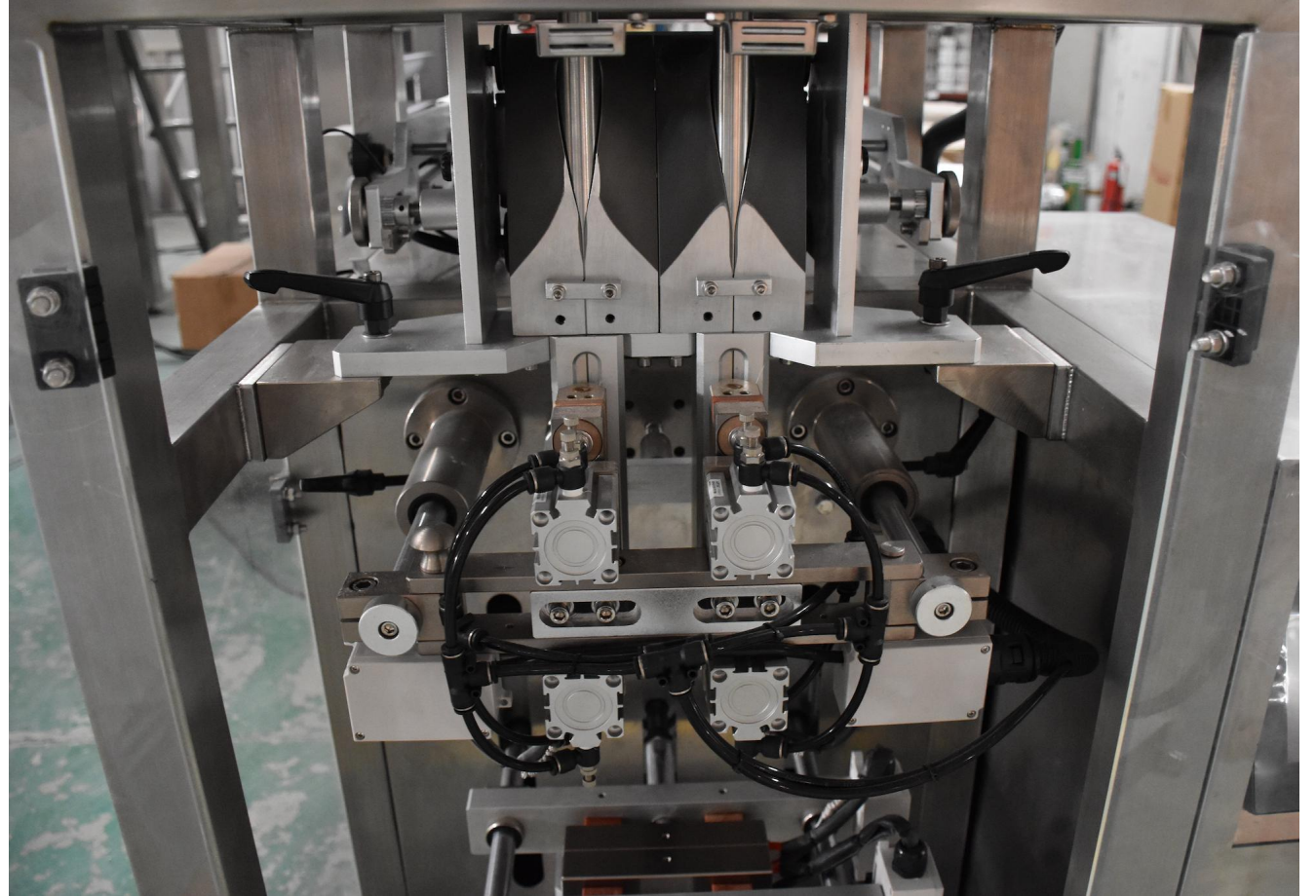
Vertical Sealing and Bag former
