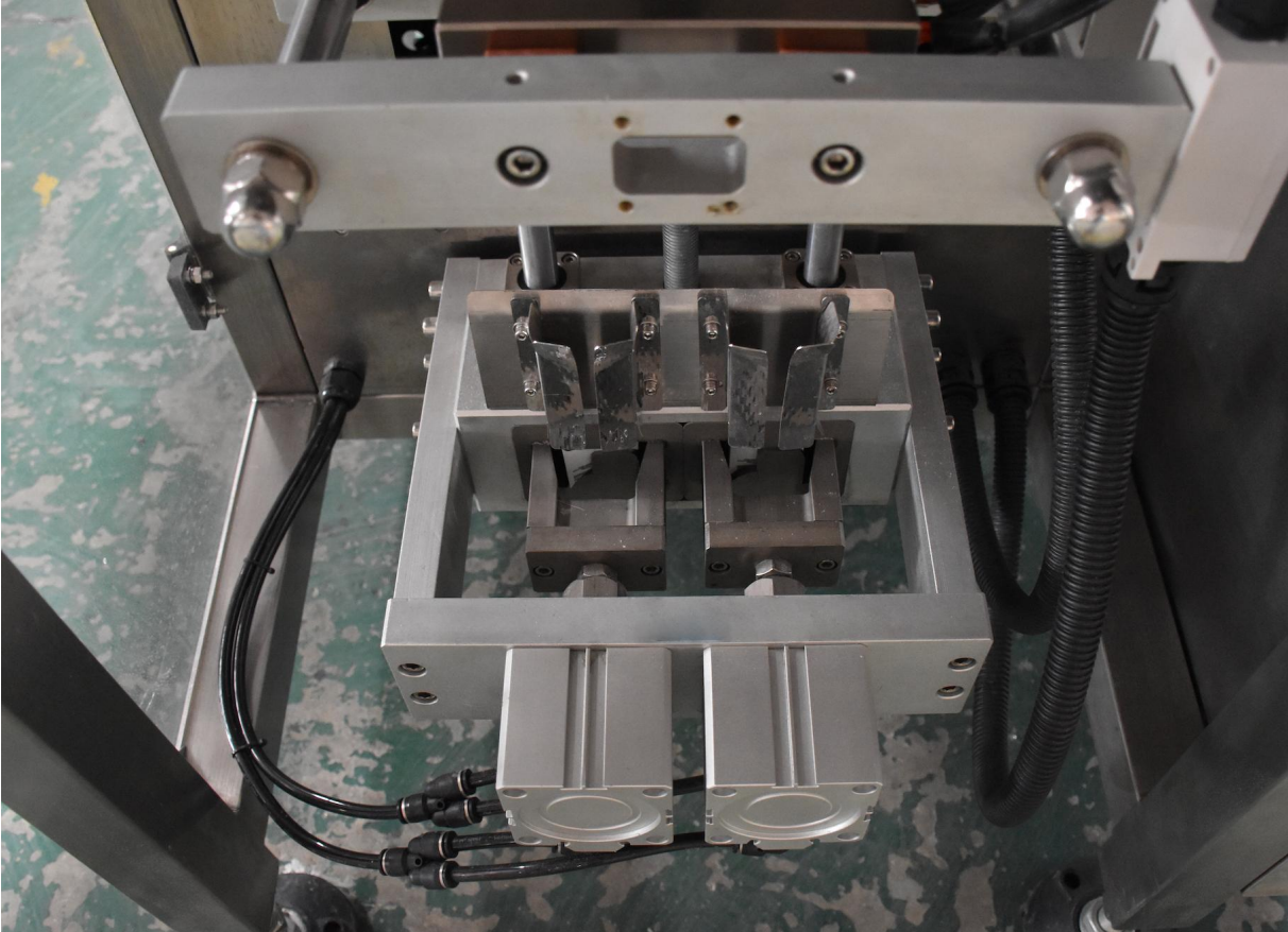
Horizontal Sealing and Cutting
